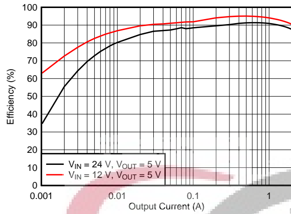
Figure 17. Efficiency
